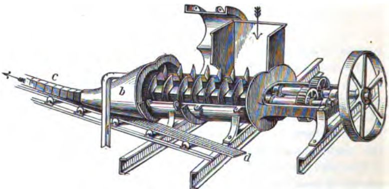
Fig. 399.—Cutting cylinder of Grotjahn's machine.
